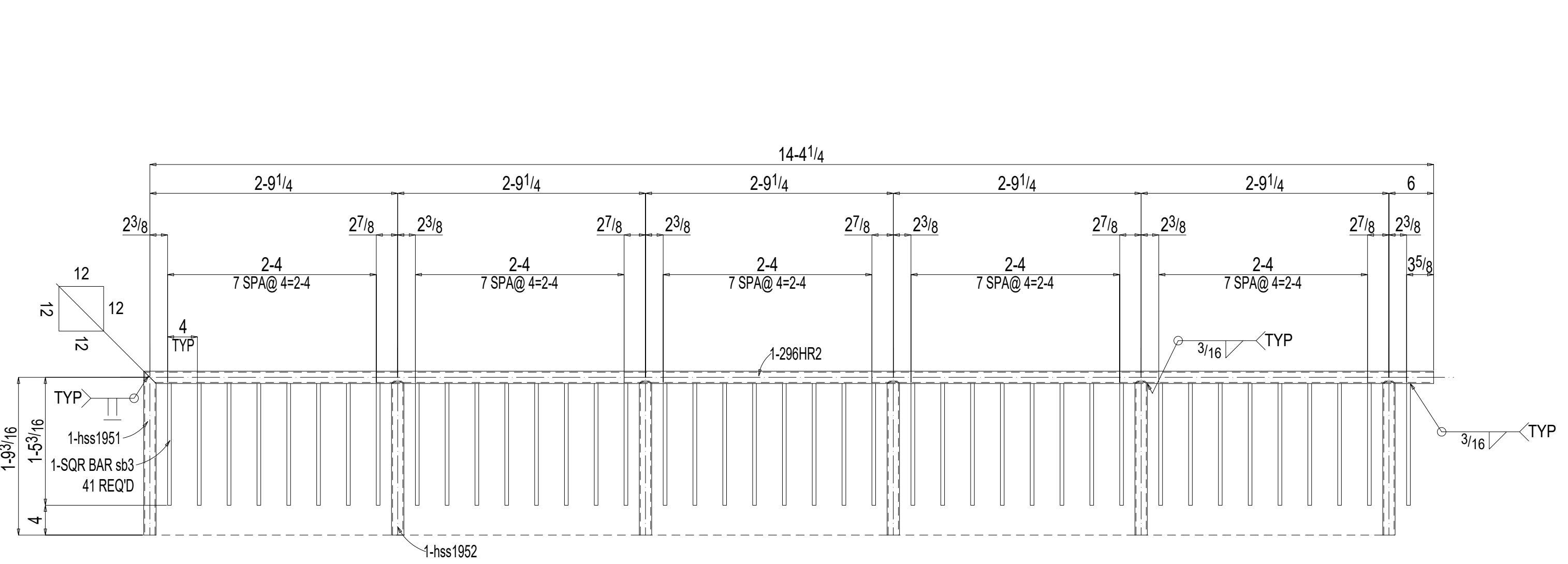
ONE HANDRAIL 296HR2
