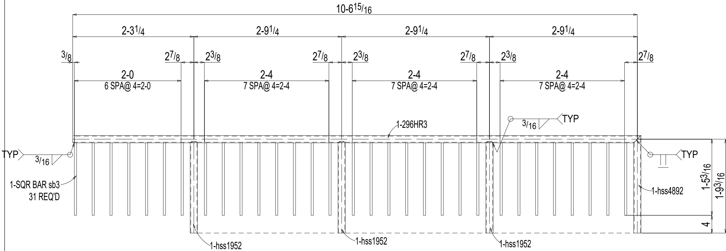
ONE HANDRAIL 296HR3
