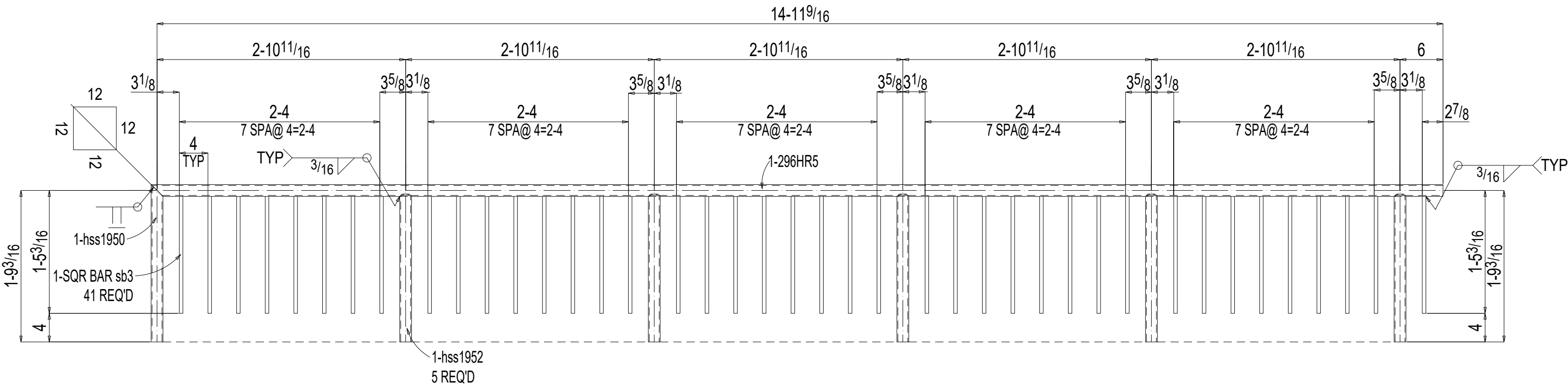
ONE HANDRAIL 296HR5
