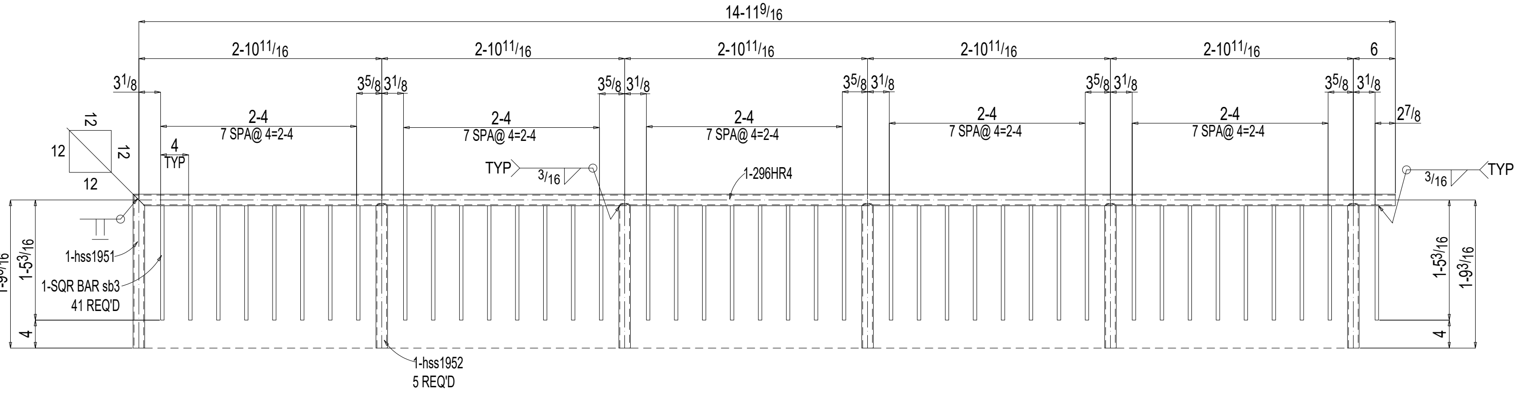
ONE HANDRAIL 296HR4
