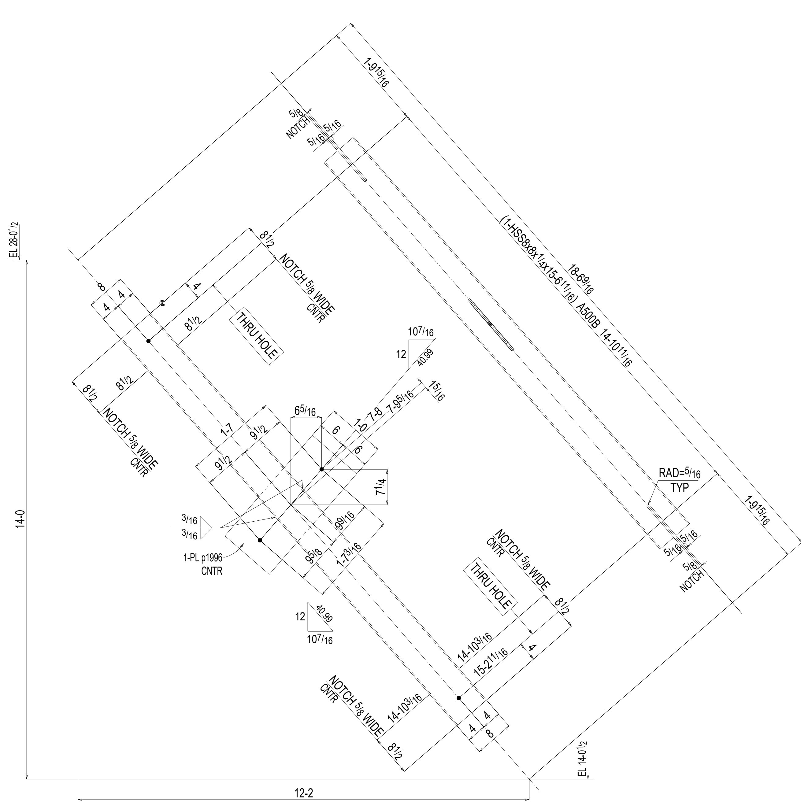
ONE VERTICAL BRACE 271VB1
