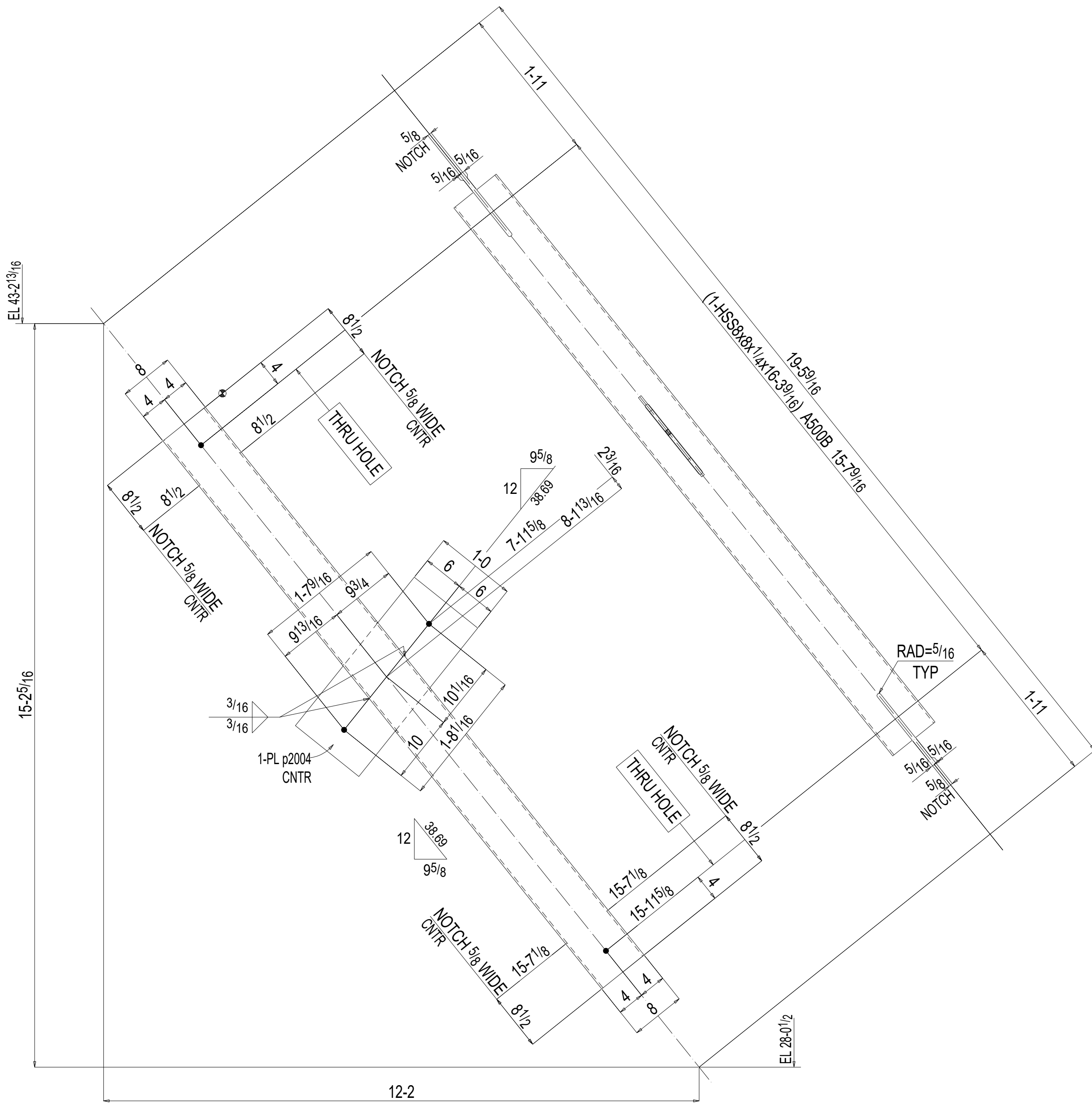
ONE VERTICAL BRACE 271VB2
