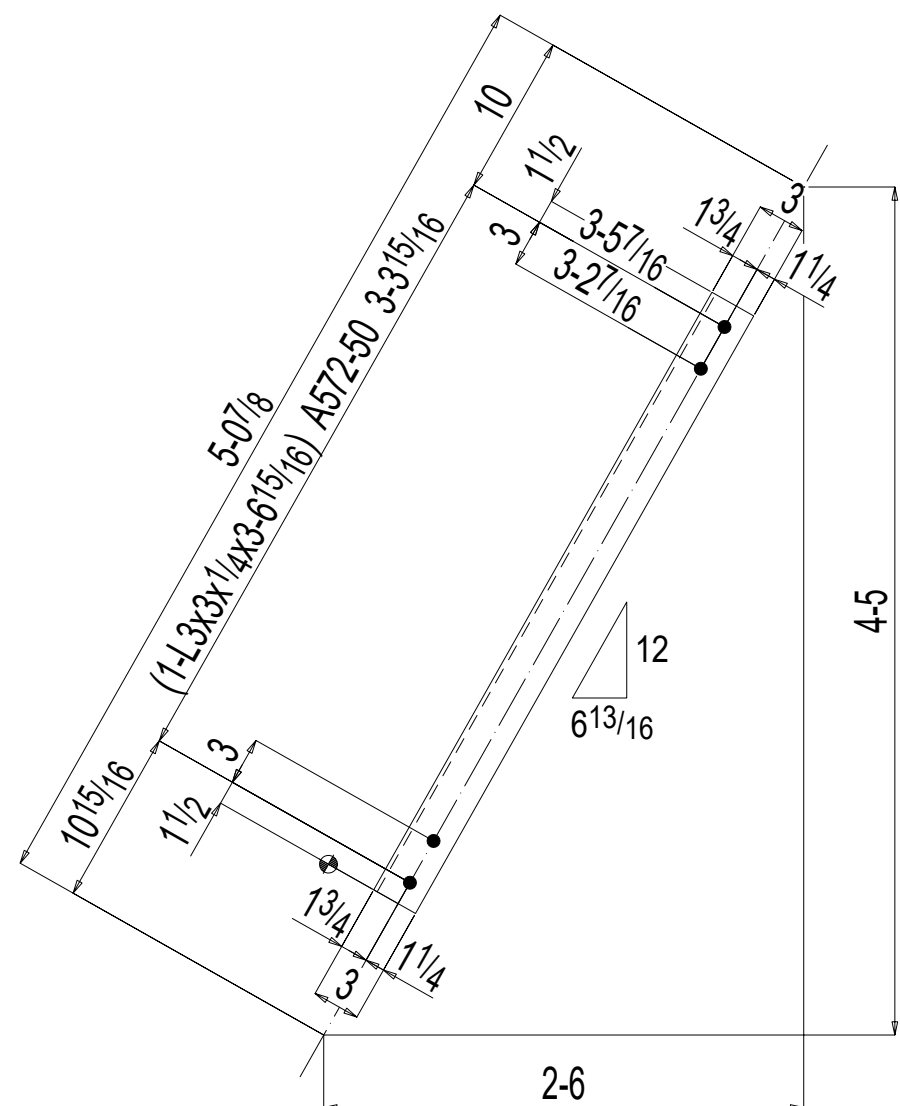
2 HORIZONTAL BRACES 28HB8
