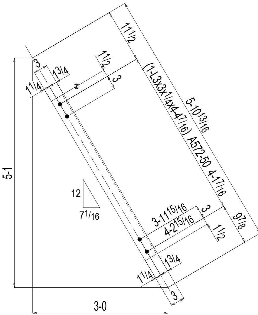
ONE HORIZONTAL BRACE 28HB7
