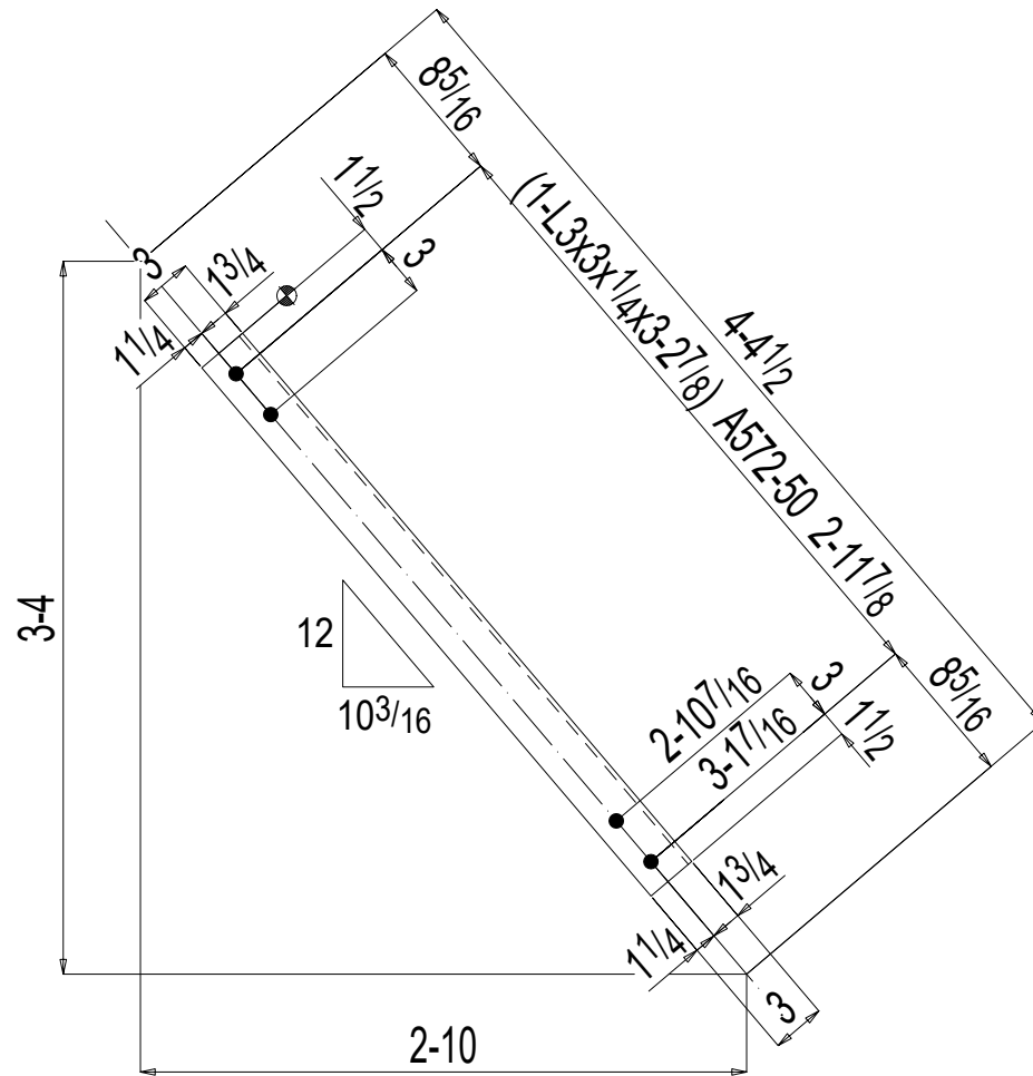
2 HORIZONTAL BRACES 28HB3
