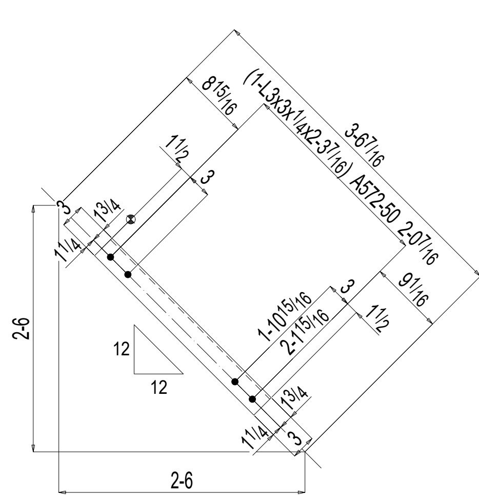
ONE HORIZONTAL BRACE 28HB1
