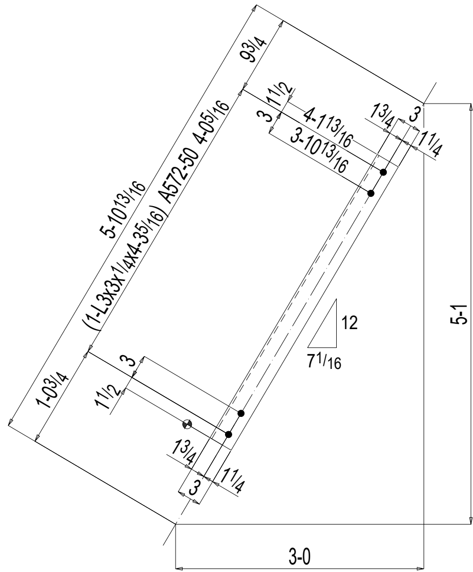
ONE HORIZONTAL BRACE 28HB6
