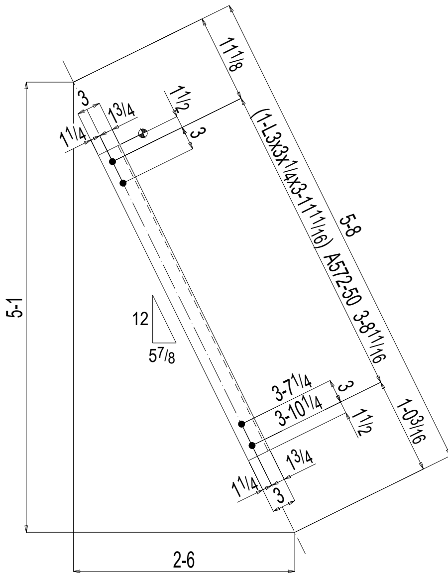
ONE HORIZONTAL BRACE 28HB5
