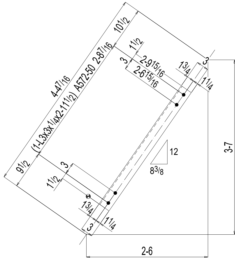
ONE HORIZONTAL BRACE 28HB4
