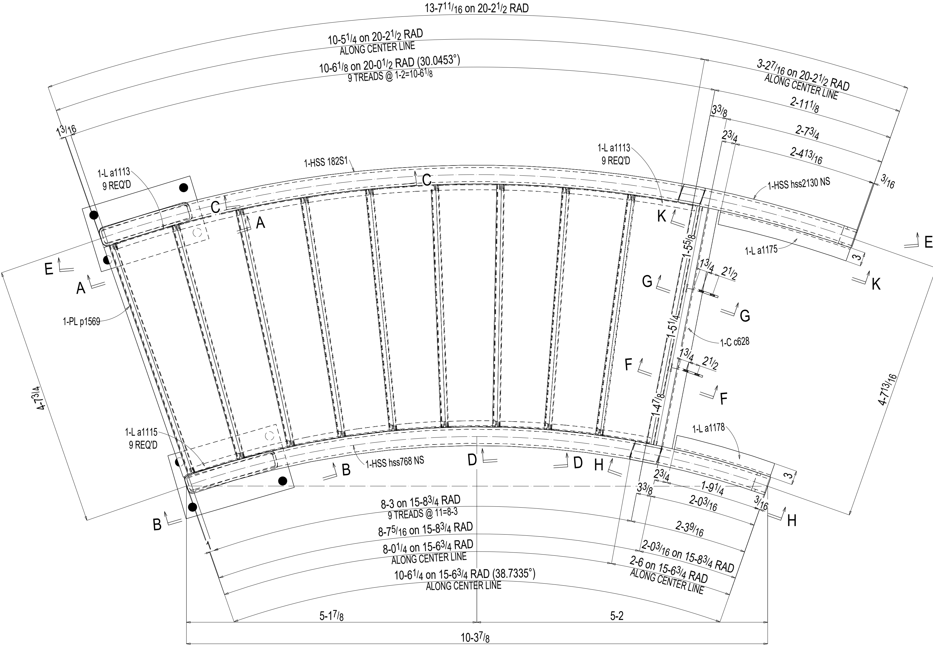
ONE STAIR 182S1
