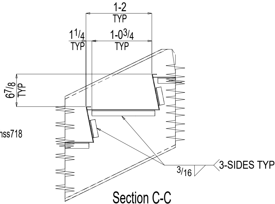
Section C-C 182S1
