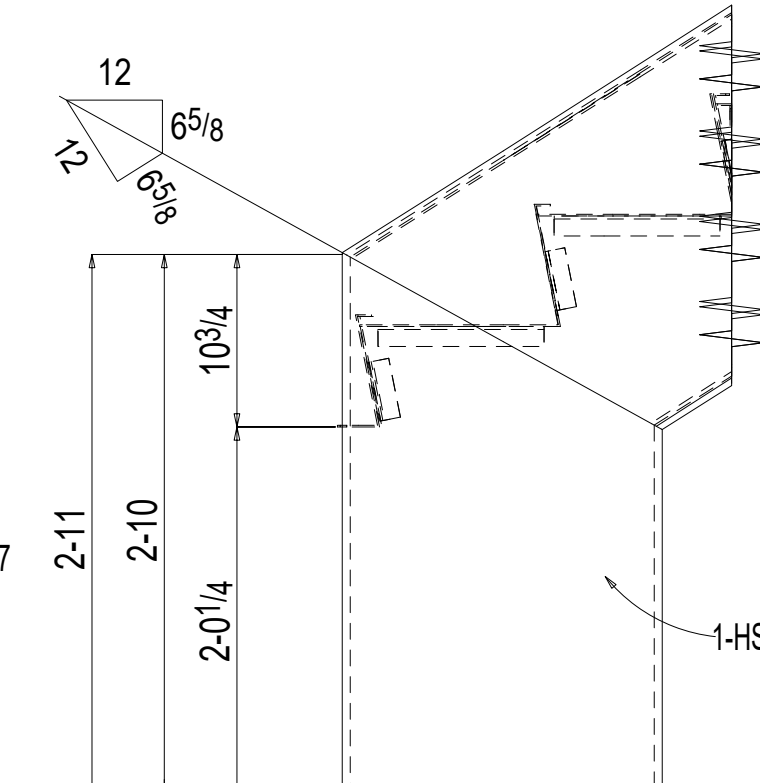
Section B-B 182S1
