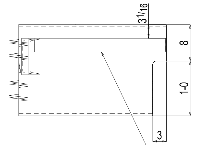
Section K-K 182S1
