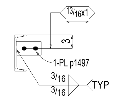
Section F-F 182S1
