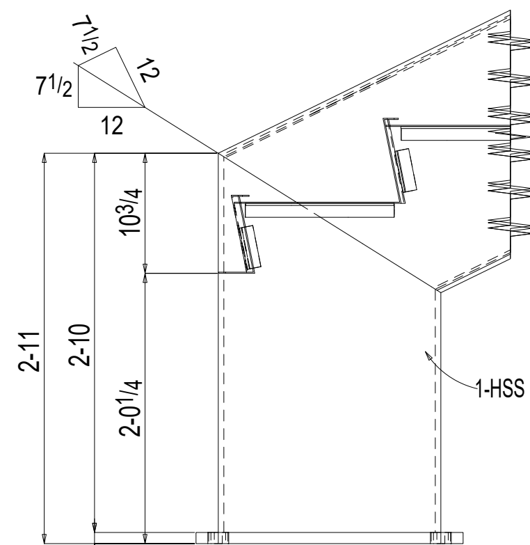
Section A-A 182S1
