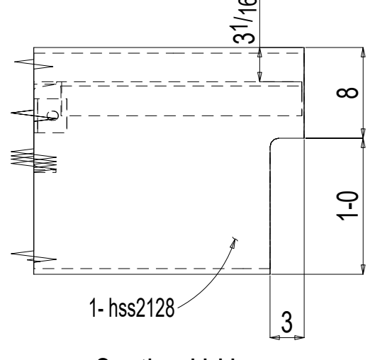
Section H-H 182S1
