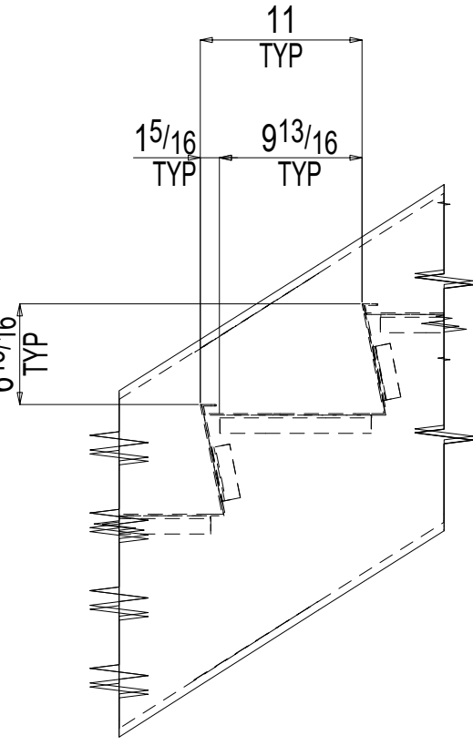
Section D-D 182S1
