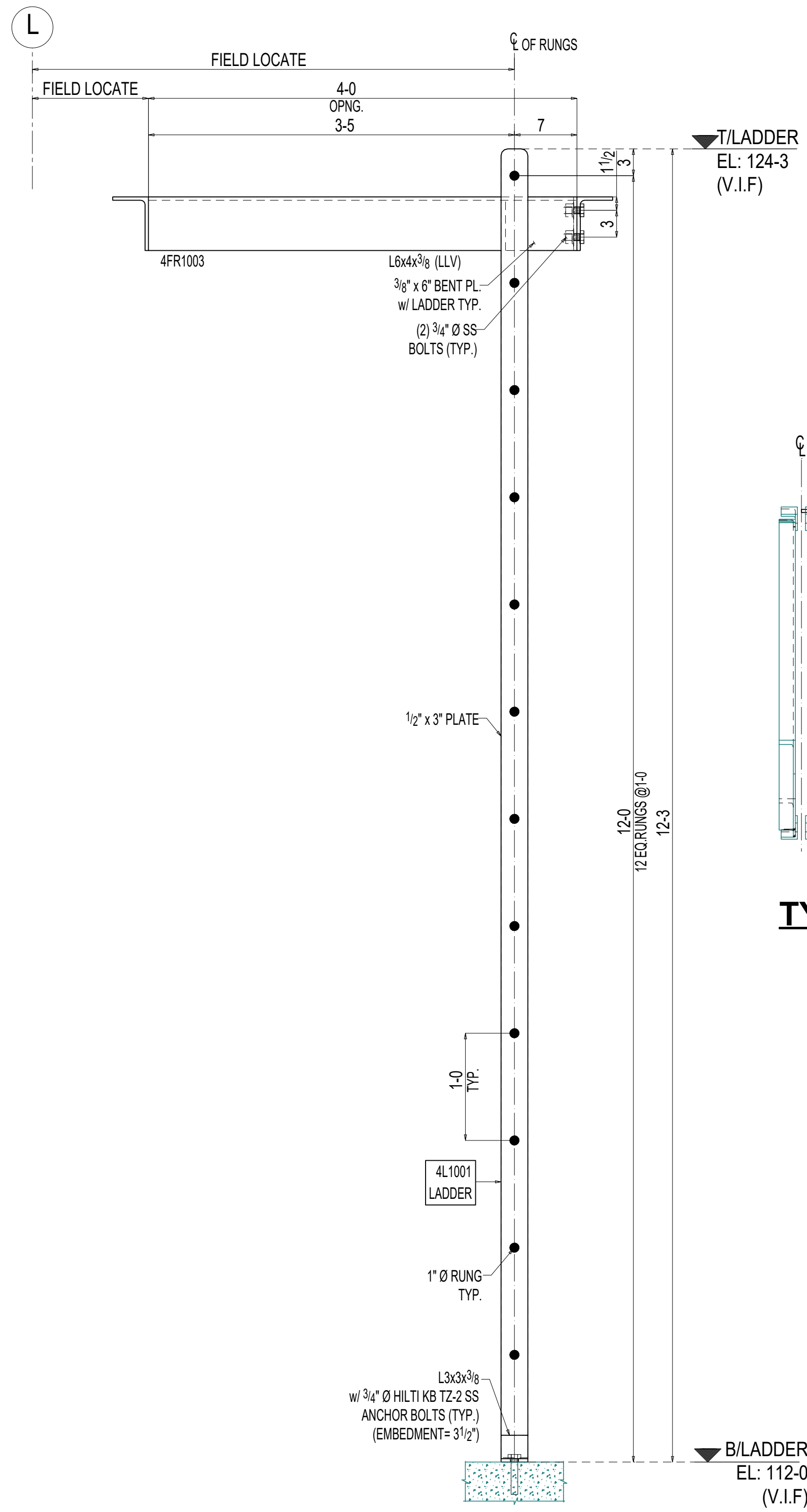
2 ELEVATION VIEW NOTE: 1) LLV = INDICATES LONG LEG VERTICAL.
