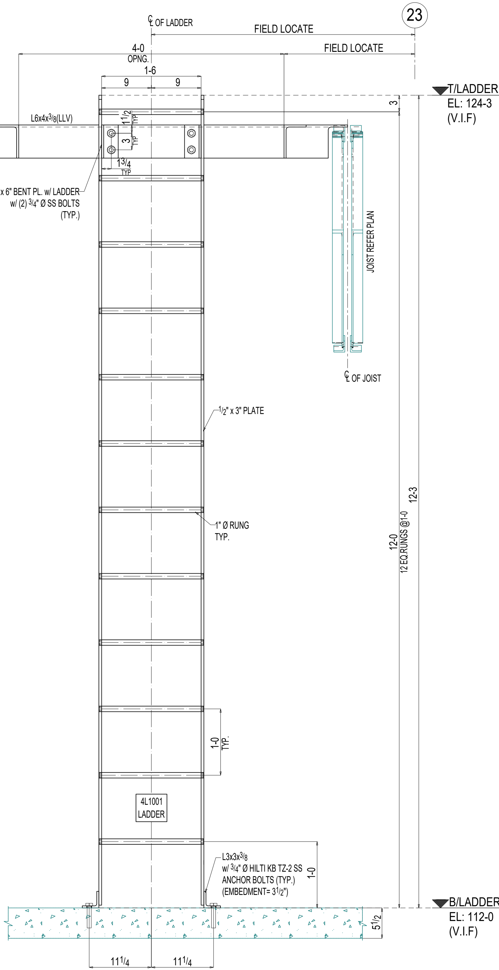
1 ELEVATION VIEW NOTE: 1) LLV = INDICATES LONG LEG VERTICAL.
