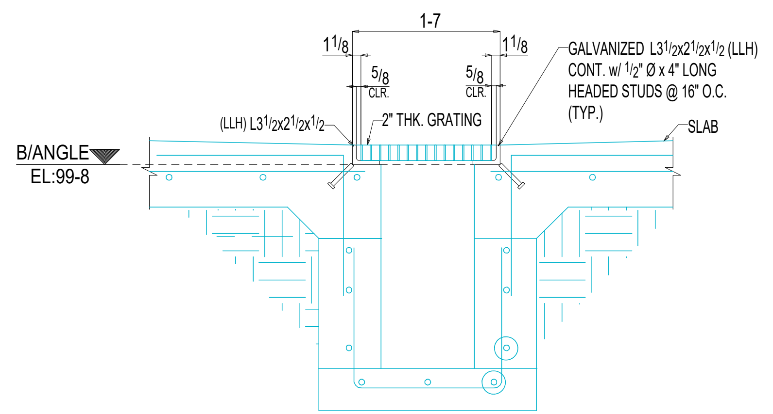
1/E2 SECTION VIEW (REF.DWG. 17/S5.1)
