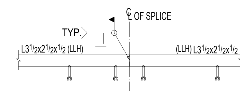
TYPICAL ANGLE SPlice CONNECTION
