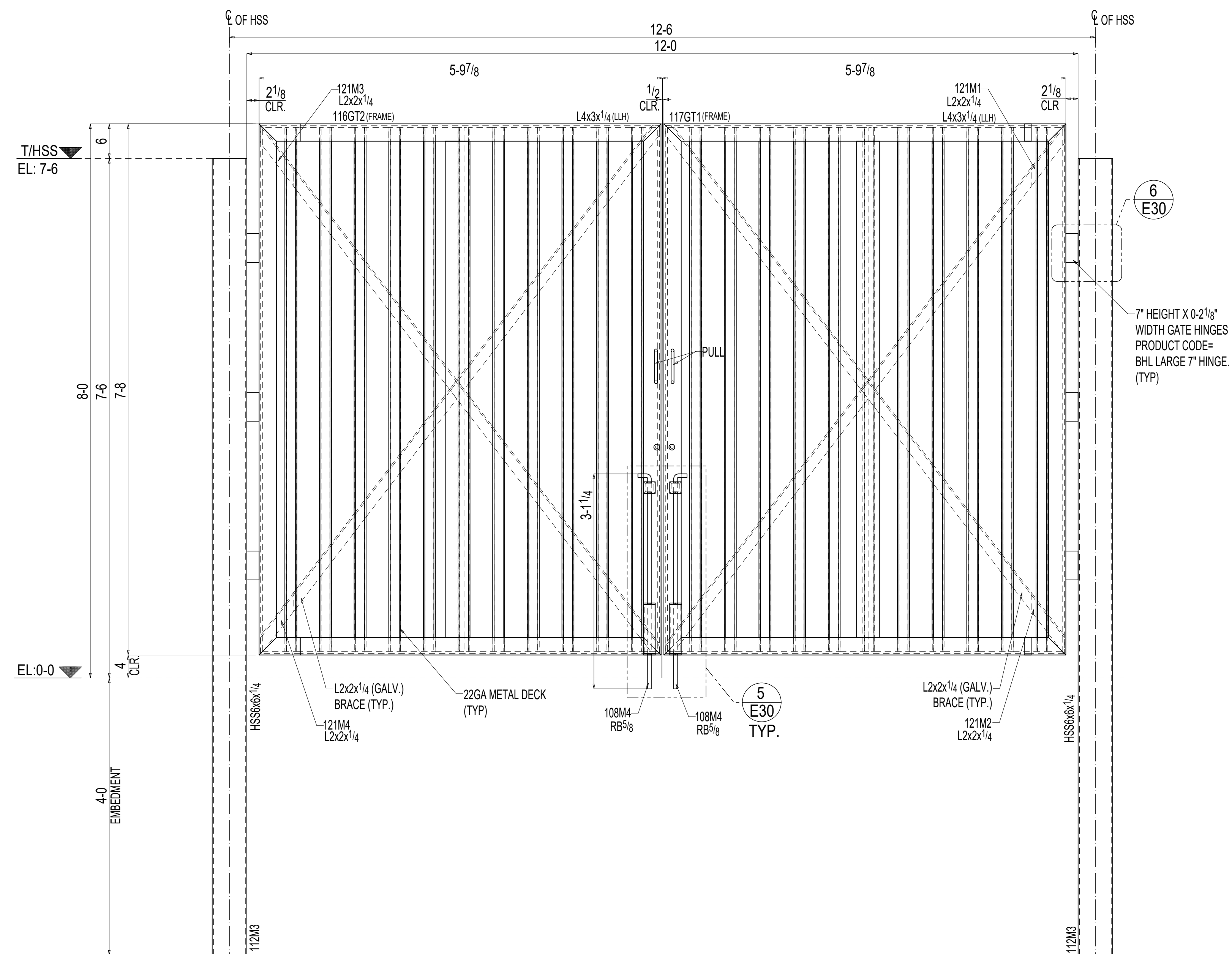
1 ELEVATION VIEW E30 (REF.DWG. 05/AS1.4)
