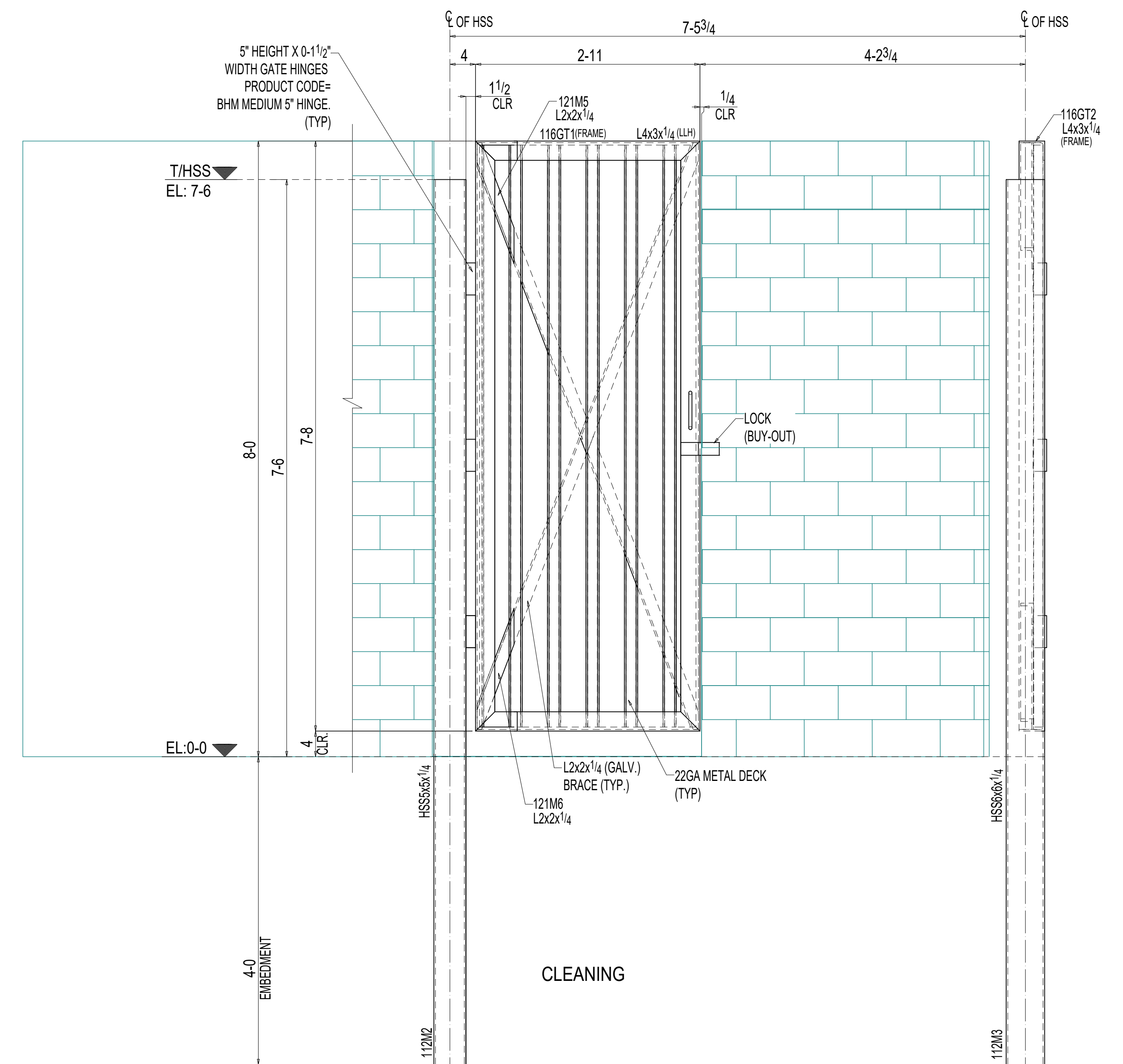
2 ELEVATION VIEW E30 (REF.DWG. 03/AS1.4)
